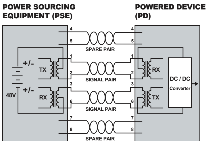
Figure 2: Power Supplied over Data Pins
