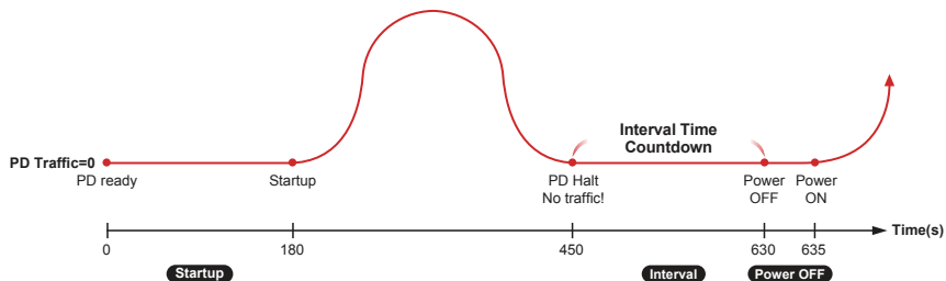
Figure 2-6: Alive Check Mechanism
