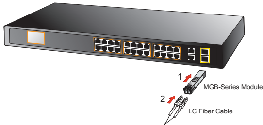
Figure 3-4: Plug In the SFP Transceiver
