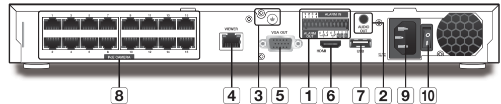
QRN-1610S
