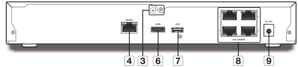
QRN-810S
