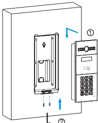
Flush Mounting
