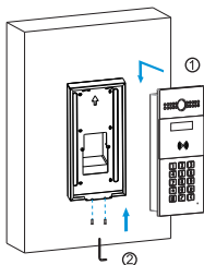
Wall Mounting
