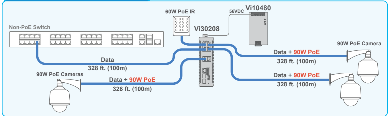
The Vi30208 and Vigitron Hardened power supplies can power multiple high power PoE PTZ Cameras up to 90W.
