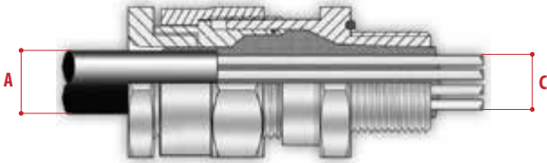
Barrier cable gland with unarmoured cable
