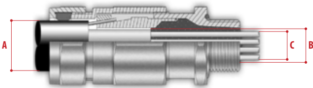
Barrier cable gland with armoured cable
