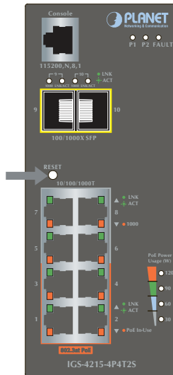
Figure 10-1: IGS-4215-4P4T/IGS-4215-4P4T2S Series Reset Button
